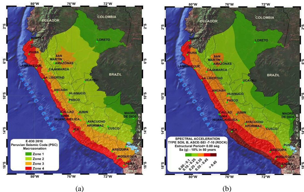
Fig. 8 – Peruvian Seismic Macrozonation Map. (a) PSC E-030, 2016; (b) This study
