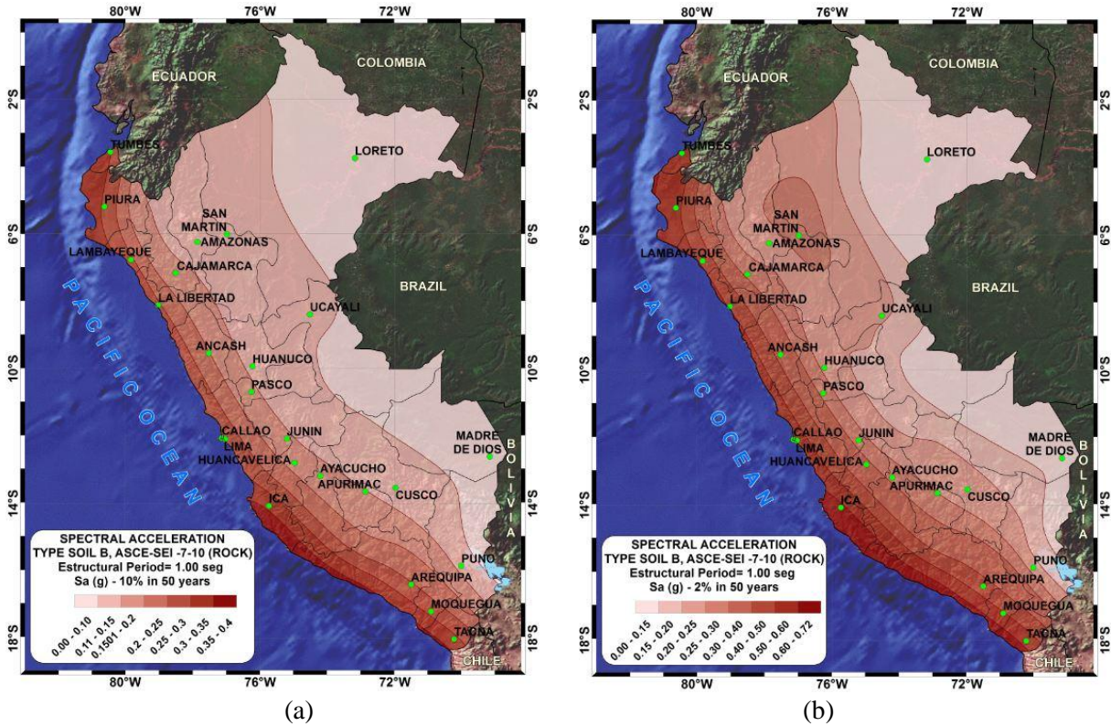
Fig. 7 – Spectral Acceleration Maps for 1.0 s. (a) 475 year return period; (b) 2475 year return period
