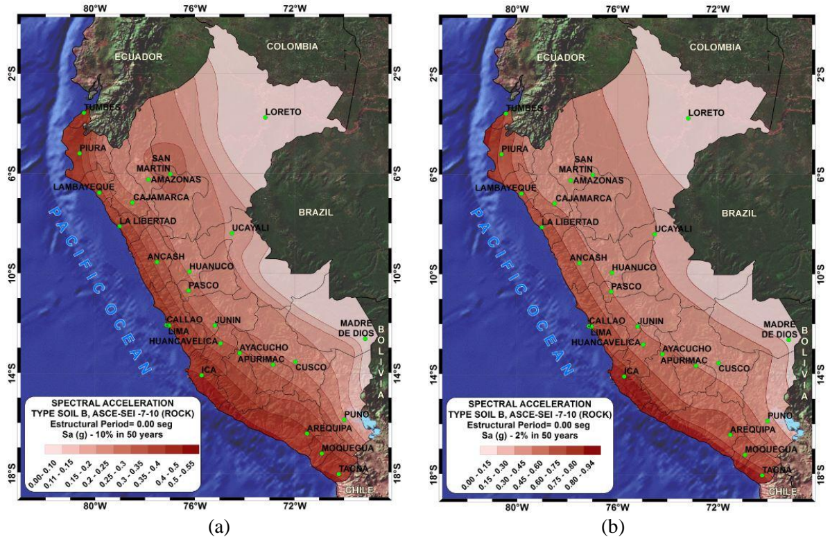
Fig. 5 – Spectral Acceleration Maps for 0.0 s (PGA). (a) 475 year return period; (b) 2475 year return period
