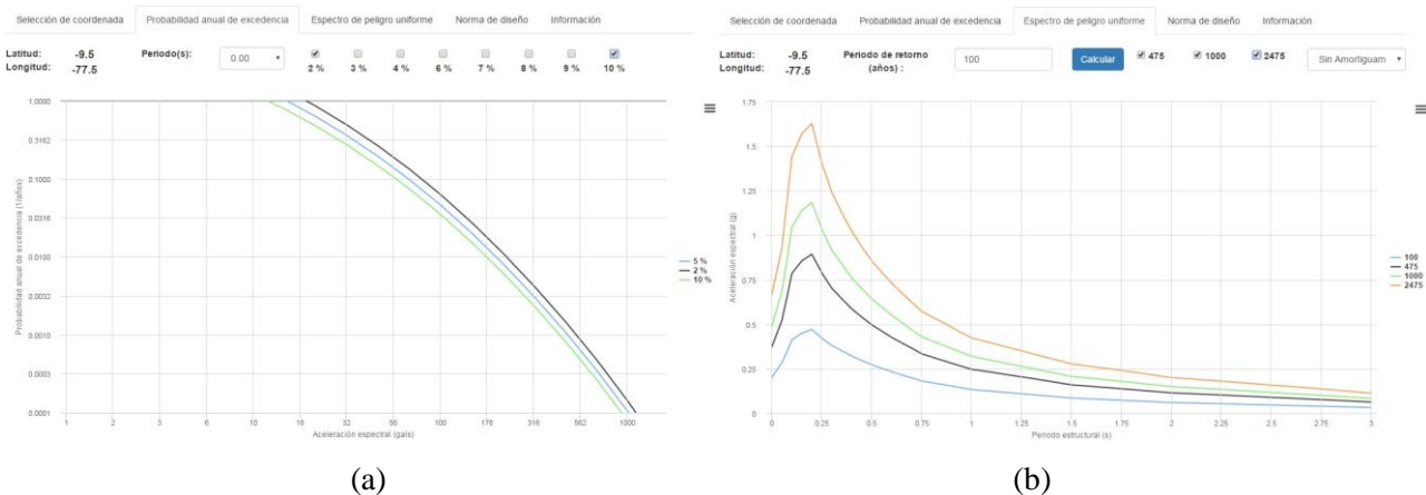
Fig. 10 – Web application output. (a) Annual Frequency of Exceedance vs Spectral Acceleration. (b) Uniform Hazard Response Spectra
