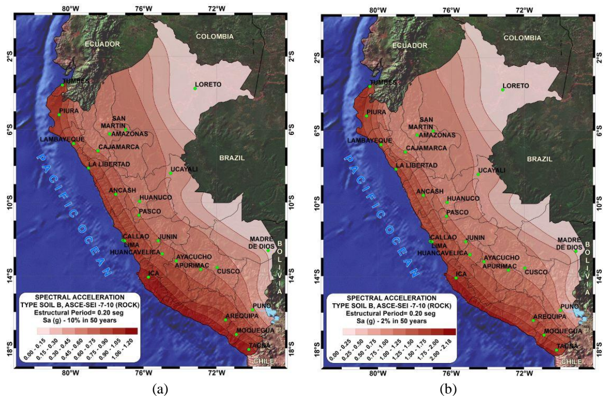
Fig. 6 – Spectral Acceleration Maps for 0.2 s. (a) 475 year return period; (b) 2475 year return period
